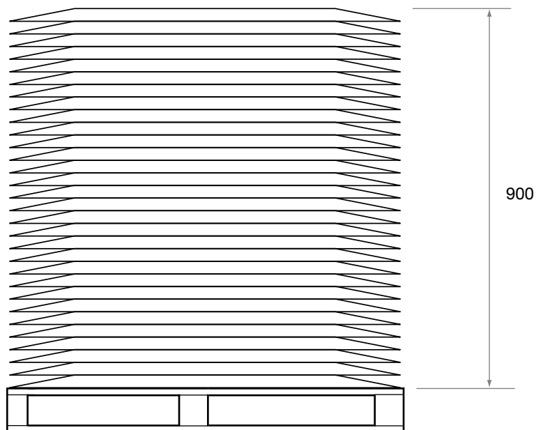
30 SAFE COVER ON PALLET
